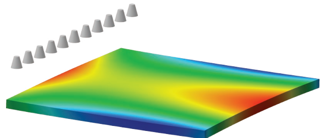
Thermo-elastic-plastic problem simulation. Distribution of vertical displacement shows distortion of the quenched steel sheet
