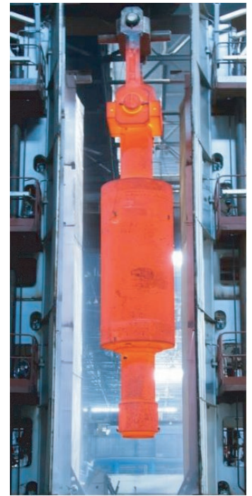
Quenching of the rotor in the sprayer device
