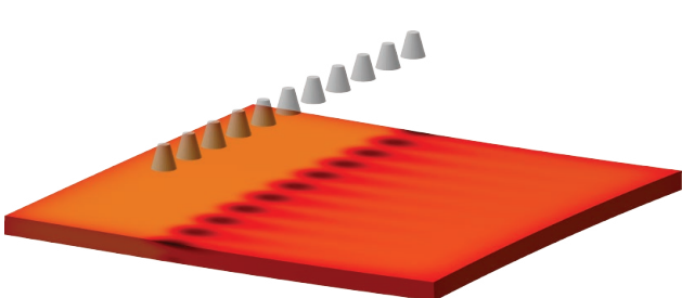
A special type of boundary conditions for spray quenching simulation. Temperature distribution is shown
